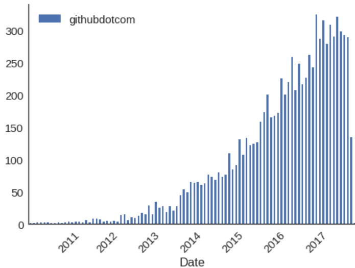
References to GitHub repositories in papers indexed in EuroPMC
